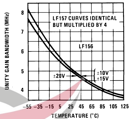
Figure 14. Gain Bandwidth
