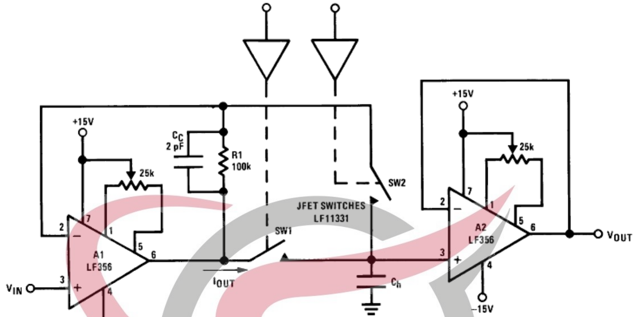
Figure 51. Fast Sample and Hold
