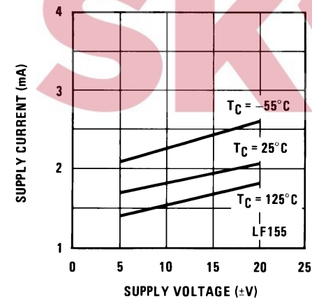
Figure 5. Supply Current
