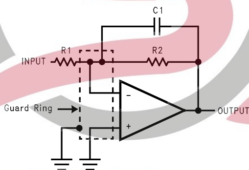
Figure 58. Inverting Amplifier
