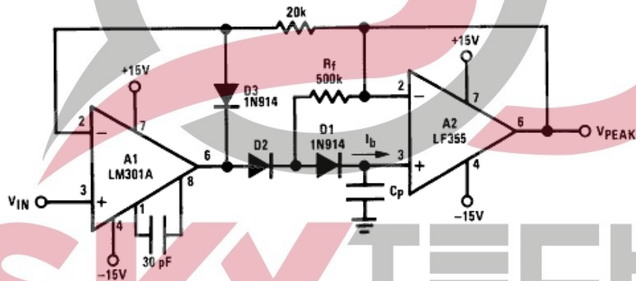
Figure 47. Low Drift Peak Detector
