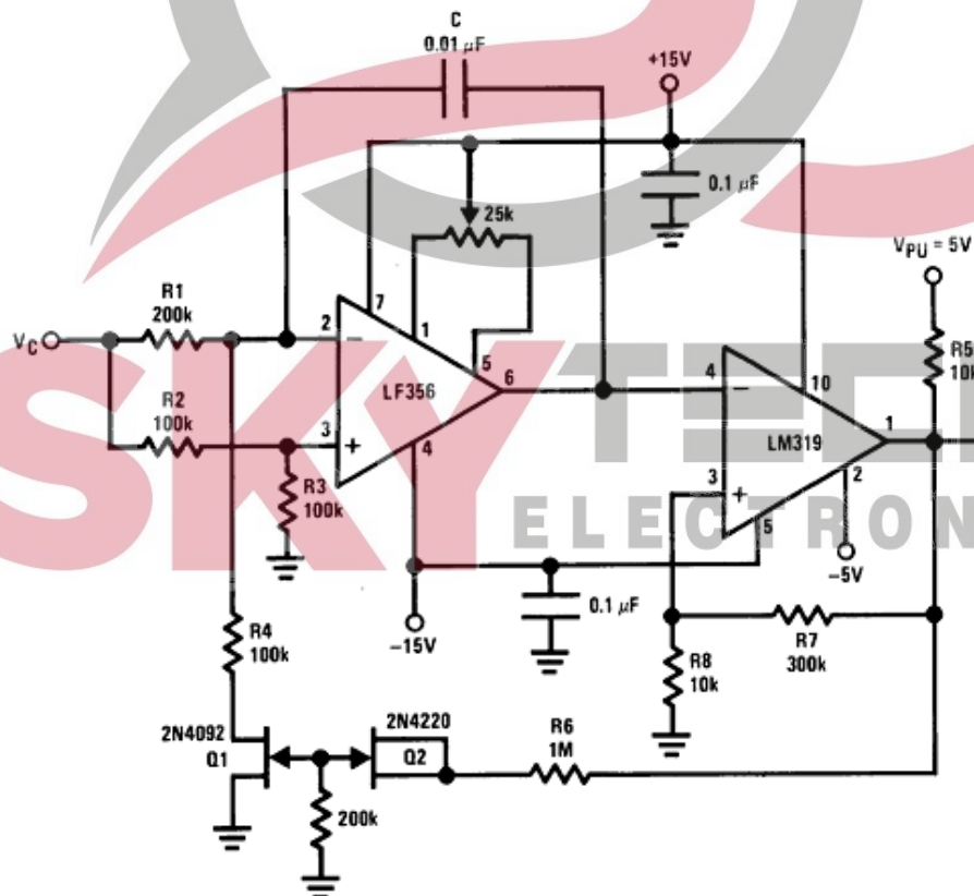
Figure 45. Decades VCO
